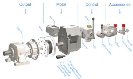
Armak Air Motor Modular System
